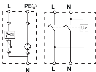
COMBI-2PT12,5/50
