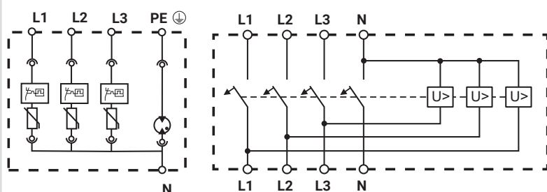
COMBI-4PT12,5/50
