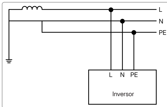
Figura 4-6 TN-C-S
