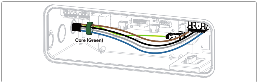
AC Terminals
