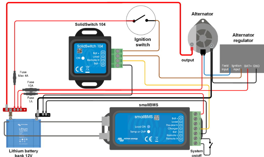
Example diagram 1: SolidSwitch 104 used with a smallBMS, to control the alternator
