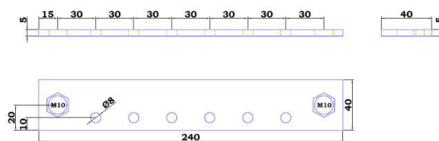
CIP100400070 = Busbar to connect 6 CIP100200100
