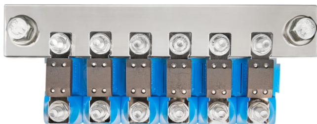
Stacked fuse holders with 6-position high current bus bar (copper 40 x 5 mm)
