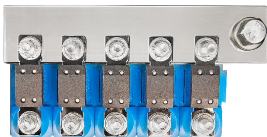
Stacked fuse holders with 5-position high current bus bar (copper 40 x 5 mm)
