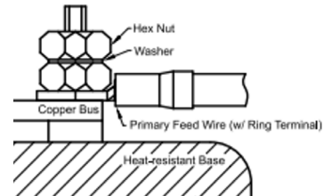
Recommended mounting
