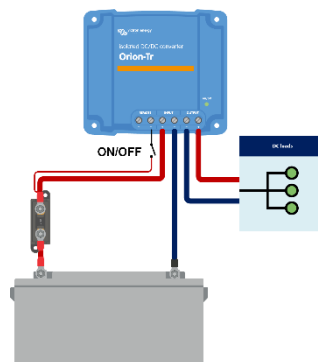
ON/OFF switch connected to battery plus
