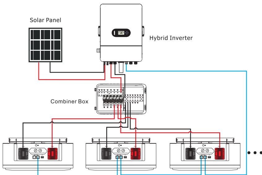
Figure 3-2 Multiple Battery Parallel System Connection Diagram
