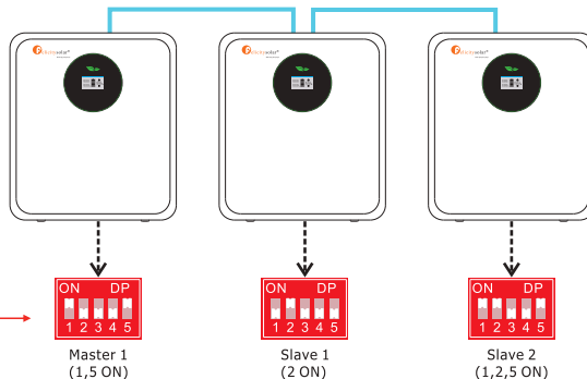
Example of three batteries in parallel
