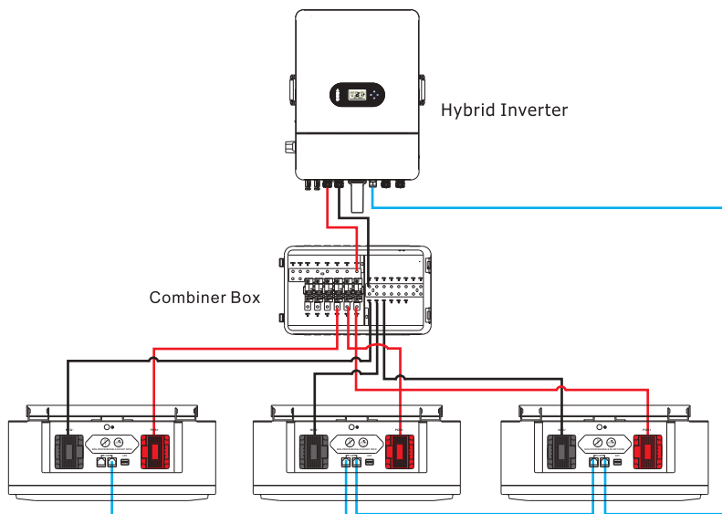
Figure 4-1 The parallel connection of three battery packs
