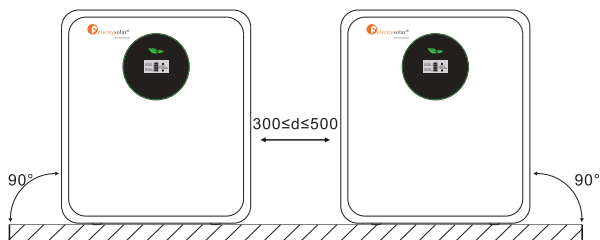
Ground(Two rows installtion)
