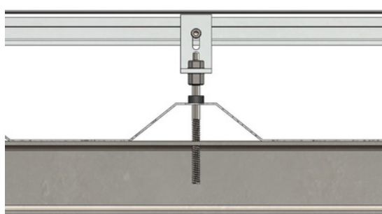
Hanger bolt
