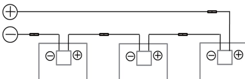
Fig. 10-1 Series Connection
