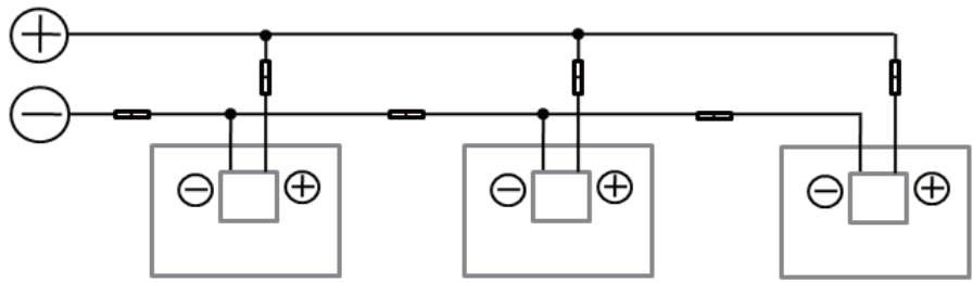
Fig.10-2 Parallel Connection
