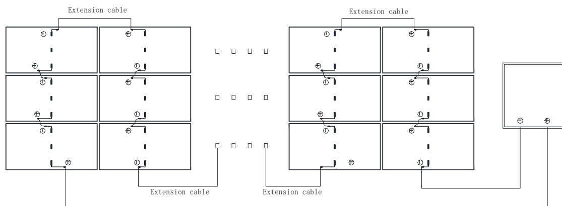
Fig. 9-2 Horizontal installation of short cable modules
