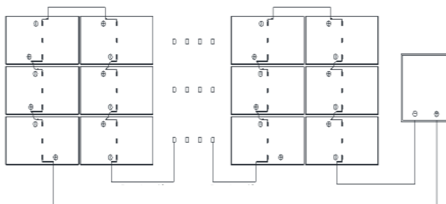
Fig. 9-4 Horizontal installation of long cable modules
