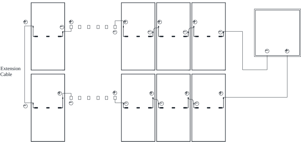
Fig. 9-1 Vertical installation of short cable modules
