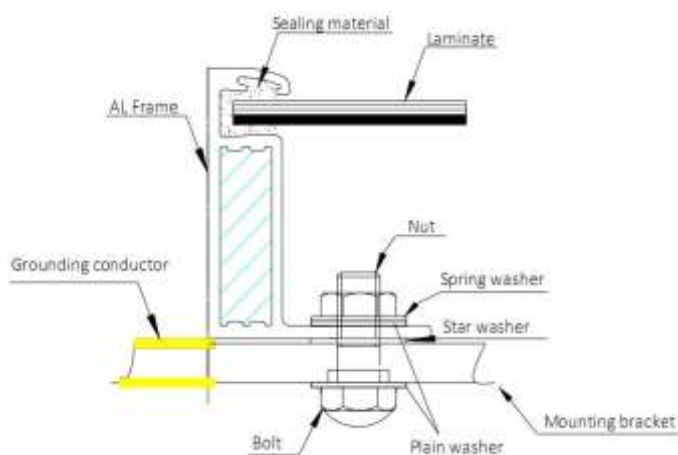
Fig. 11.1 M5 Pan head screw grounding
