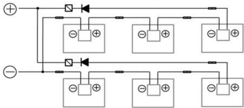
Fig.10-3 Parallel-series Connection
