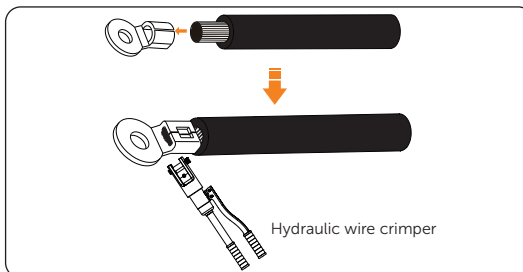
Figure 7-8 Crimping terminal
