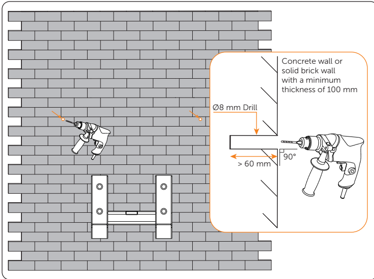
Figure 6-15 Drilling holes
