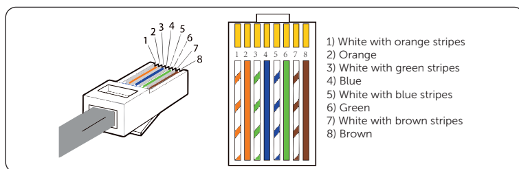
Figure 7-5 Wire sequence
