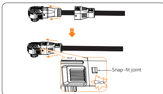
Figure 7-14 Assembling connector
