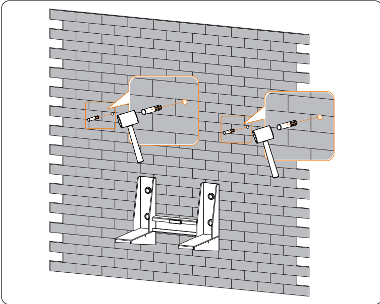
Figure 6-16 Insert expansion bolts
