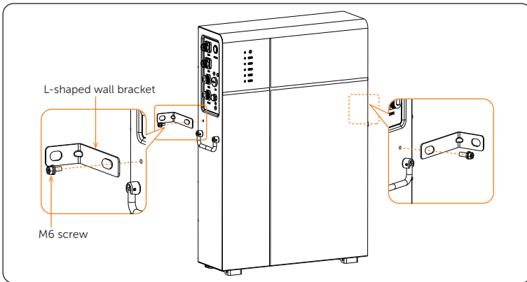
Figure 6-12 Fixing L-shaped wall bracket to the battery pack
