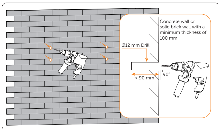
Figure 6-10 Drawing holes
