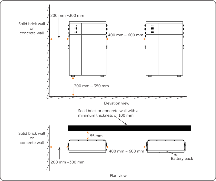
Figure 4-3 Clearance requirement about wall mounting
