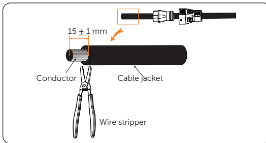
Figure 7-12 Stripping cable jacket
