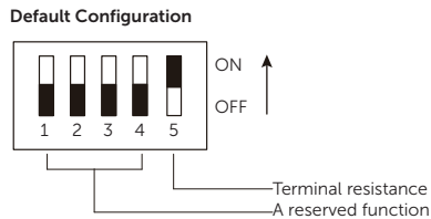
Figure 2-7 Default configuration
