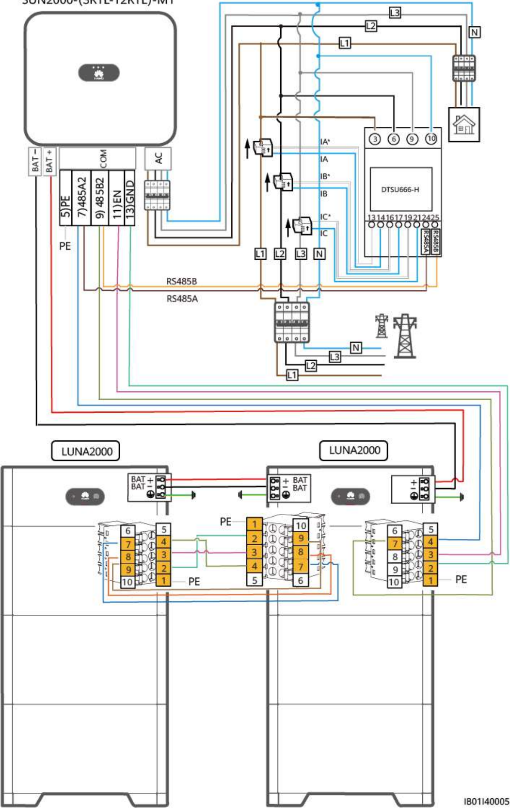
Figura 5-7 SUN2000-(3KTL-12KTL)-M1 SUN2000-(3KTL-12KTL)-M1
