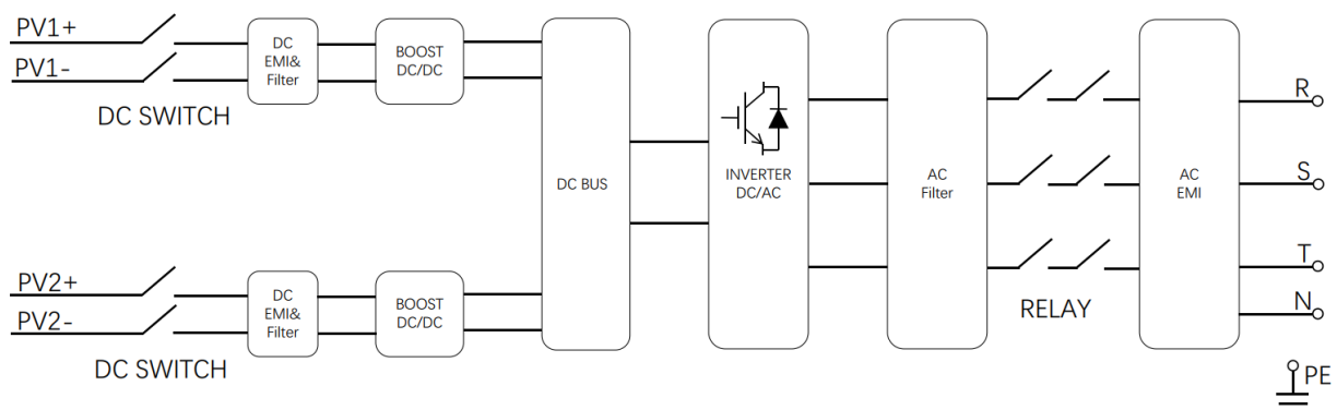
Circuit Diagram
